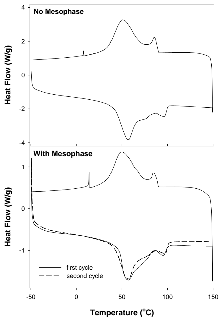
FIGURE 3. DSC thermograms of regioirregular poly(3-docosyl-thiophene). Top: slowly cooled sample containing no mesophase. Bottom: rapidly cooled sample containing the trapped mesophase. Endotherms are down and all data were collected at 10 °C/min.
