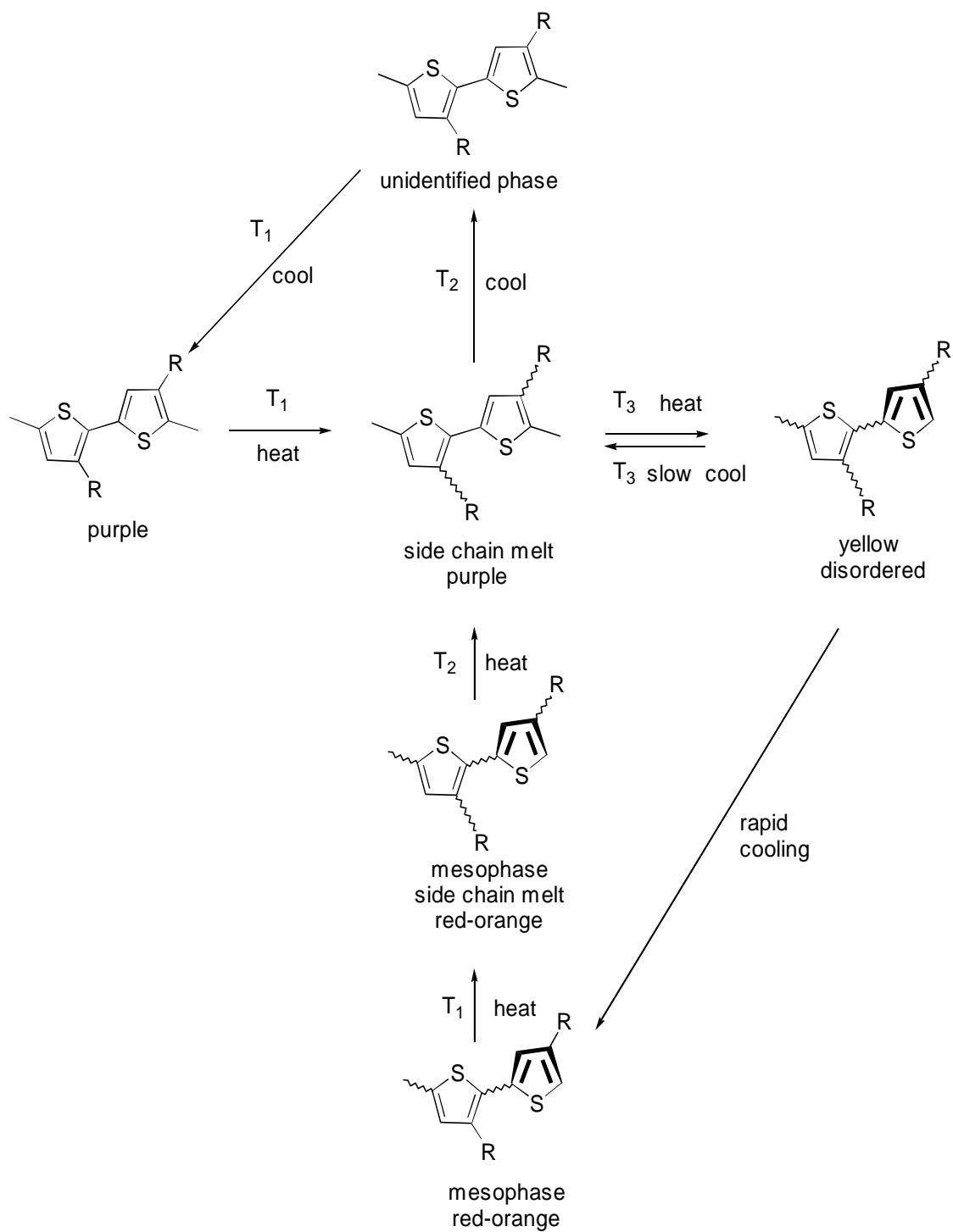
SCHEME1. Proposed Mechanism for Novel Thermochromic Properties
