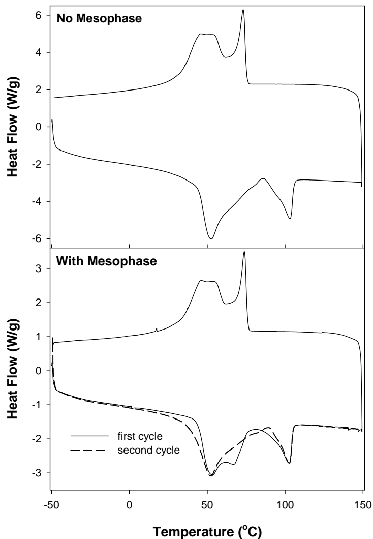
FIGURE 2. DSC thermograms of regioregular poly(3-docosyl-thiophene). Top: slowly cooled sample containing no mesophase. Bottom: rapidly cooled sample containing the trapped mesophase. Endotherms are down and all data were collected at 10 °C/min.
